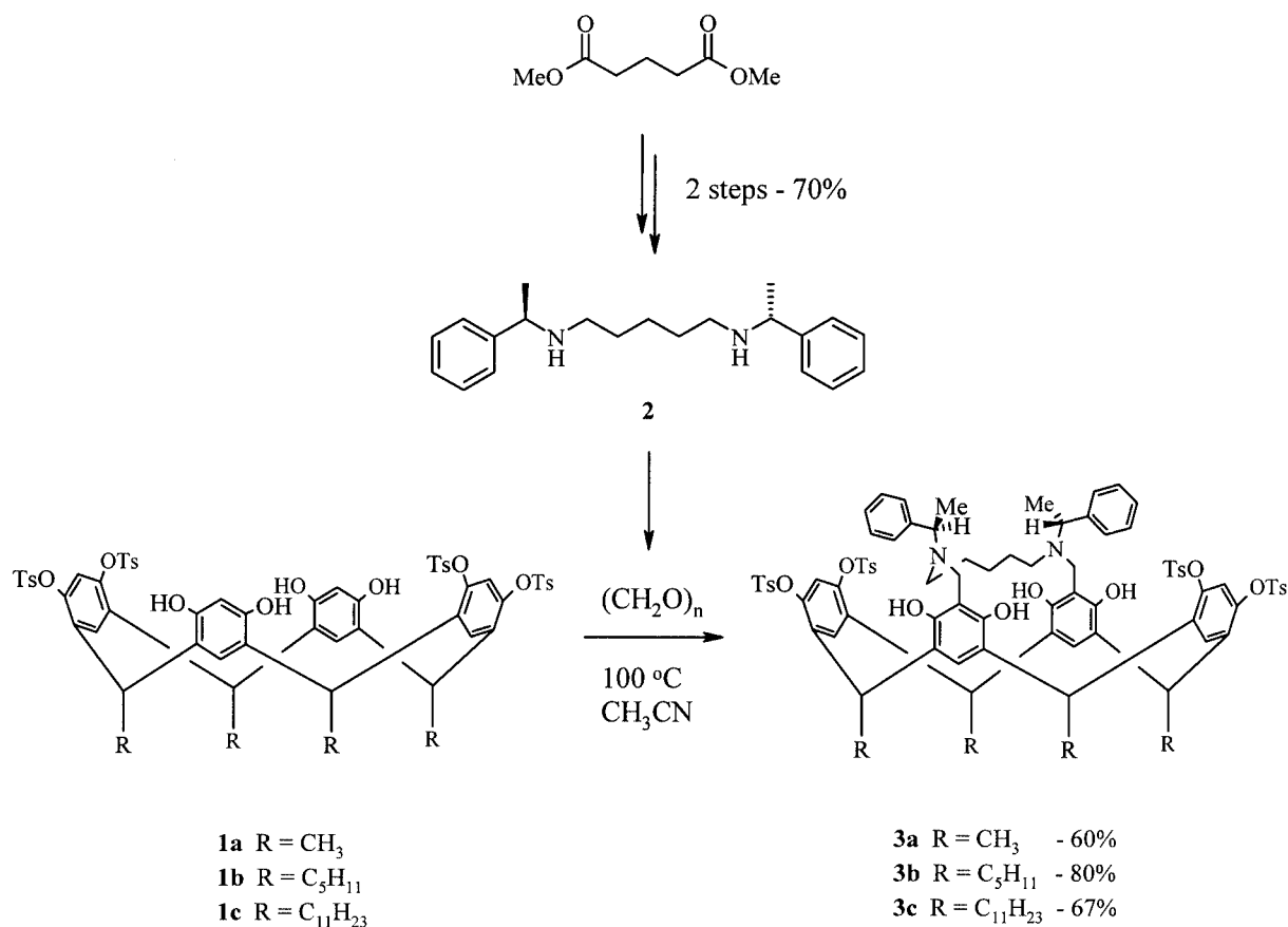
Scheme 1. General synthesis of bridged resorcinarenes
