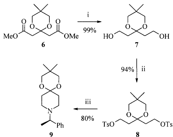
Scheme 4. Reagents and conditions: i) \text{LiAlH}_4 , THF, 0\text{ }^{\circ}\text{C} ; ii) \text{TsCl} , \text{Et}_3\text{N} , DCM, room temp.; iii) \alpha -methylbenzylamine, \text{CH}_3\text{CN} , 50\text{ }^{\circ}\text{C}
