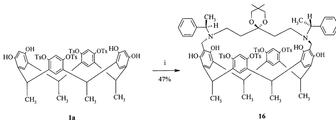
Scheme 7. Reagents and conditions: i) diamine 15 , (CH 2 O) n , CH 3 CN, 85 °C
