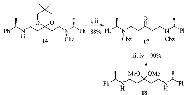
Scheme 8. Reagents and conditions: i) benzyl chloroformate, i Pr 2 NEt, DCM, 0 °C; ii) TsOH (cat), acetone, room temp.; iii) TMSOMe, TMSOTf (cat.), DCM, –20 °C; iv) Pd/C (10%), H 2 , EtOH, room temp.
