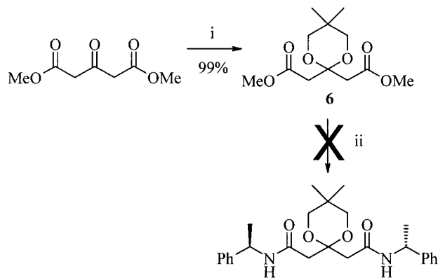
Scheme 3. Reagents and conditions: i) neopentylglycol disilyl ether, TMSOTf (cat), DCM, -20\text{ }^{\circ}\text{C} to room temp.; ii) \alpha -methylbenzylamine, 100\text{ }^{\circ}\text{C}
