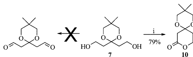
Scheme 5. Reagents and conditions: i) TPAP (5%), NMO, 4-Å sieves, DCM, room temp.
