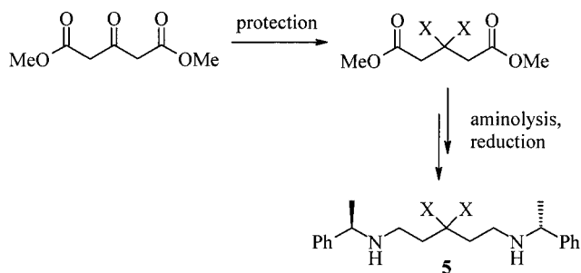
Scheme 2. Envisaged synthesis of protected functionalised diamine
