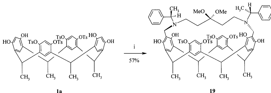
Scheme 9. Reagents and conditions: i) diamine 18 , (CH 2 O) n , CH 3 CN, 85 °C
