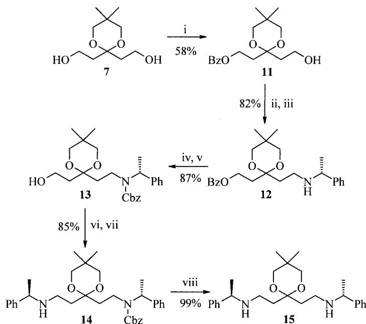
Scheme 6. Reagents and conditions: i) BzCl, Et 3 N, DCM, 0 °C to room temp.; ii) DMSO, oxalyl chloride, Et 3 N, –78 °C; iii) \alpha -methylbenzylamine, NaBH 4 , 3-A sieves, MeOH, 0 °C to room temp.; iv) Benzyl chloroformate, i Pr 2 NEt, DCM, 0 °C; v) KOH, EtOH, room temp.; vi) oxalyl chloride, DMSO, Et 3 N, DCM, –78 °C; vii) \alpha -methylbenzylamine, NaBH 4 , 3A sieves, MeOH, 0 °C to room temp.; viii) Pd/C, H 2 , EtOH, room temp.
